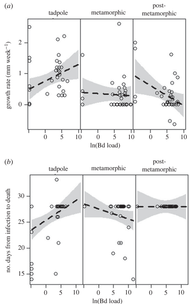
Figure 4. Host tolerance, measured as growth rate ( \text{mm week}^{-1} ; (a)) and survival (b) of Osteopilus septentrionalis as a function of the natural log of Batrachochytrium dendrobatidis abundance in tadpoles, metamorphic, and post-metamorphic frogs (from left to right). (a) There were significant effects of Bd abundance on host growth rate across life stages ( F_{2,90} = 5.15 , p < 0.01 ). Higher abundance of Bd marginally increased growth for tadpoles ( p = 0.06 ) and decreased growth for post-metamorphic frogs ( p < 0.05 ). Metamorphic frogs experienced no significant change in length across Bd abundance ( p = 0.63 ). (b) Host survival was affected by abundance of Bd across host life stage ( \chi^2_2 = 7.08 , p < 0.05 ). Days alive decreased with higher Bd abundance for metamorphic frogs ( p < 0.05 ) but was not significantly dependent on Bd abundance for tadpoles ( p = 0.29 ) and post-metamorphic frogs ( p = 1 ). Data shown as a conditional plot, with the expected value (black dashed line), a 95% confidence band for the expected value (grey band), and partial residuals (points) displayed.
